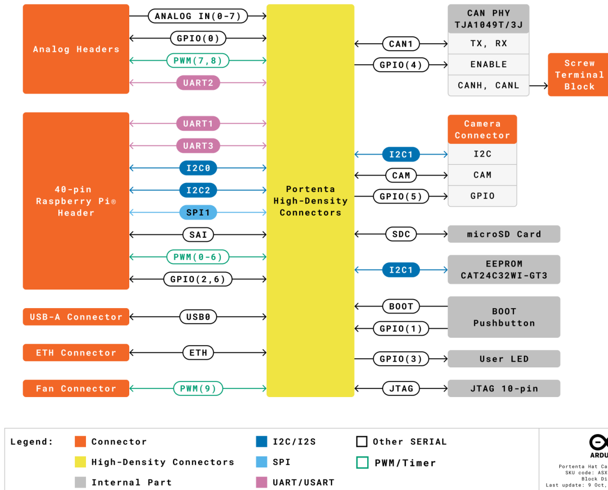
Figure 3. Portenta Hat Carrier block diagram
